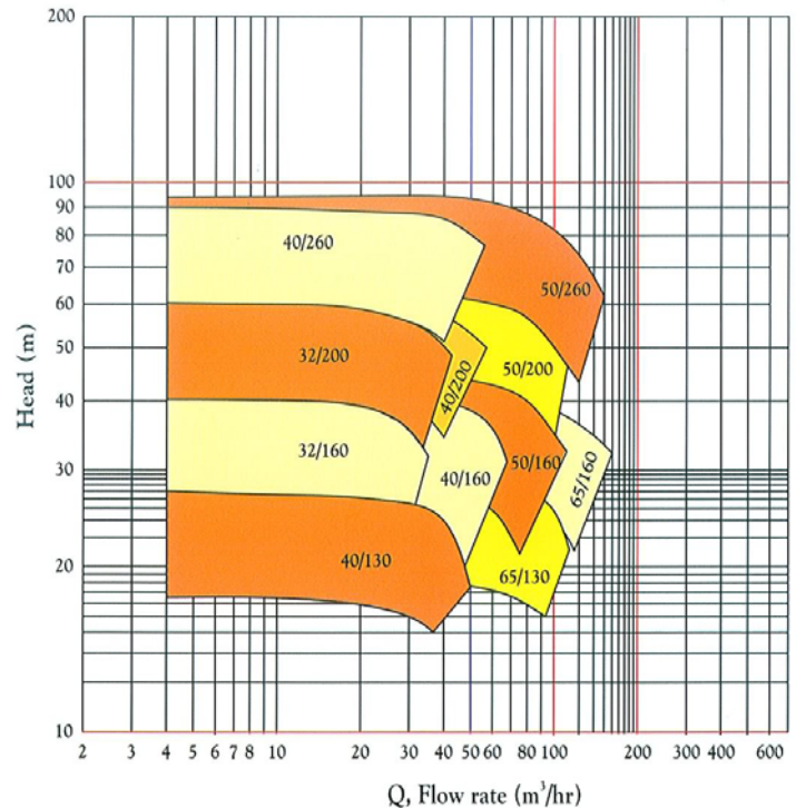
iCP Family range 2900 RPM
