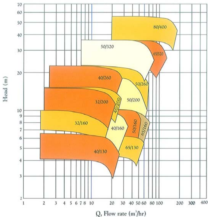
iCP Family range 1450 RPM
