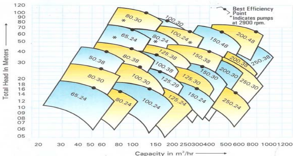
Family Curve of SCT Pumps at 1450 rpm - 50 Hz
