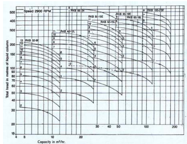
Family Curve of RKB multistage Pump at 2900 rpm - 50 Hz
