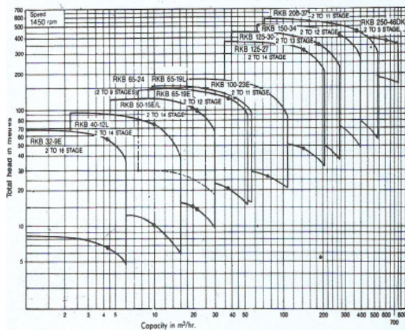
Family Curve of RKB multistage Pump at 1450 rpm - 50 Hz
