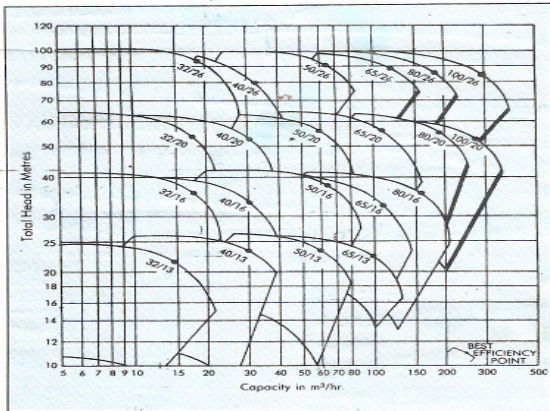
Family Curve of DB (Large size) pump at 1450 rpm – 50 Hz
