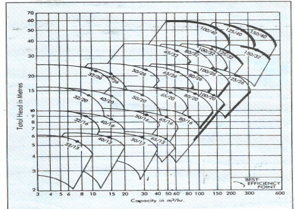
Family Curve of DB (Large size) pump at 1450 rpm – 50 Hz
